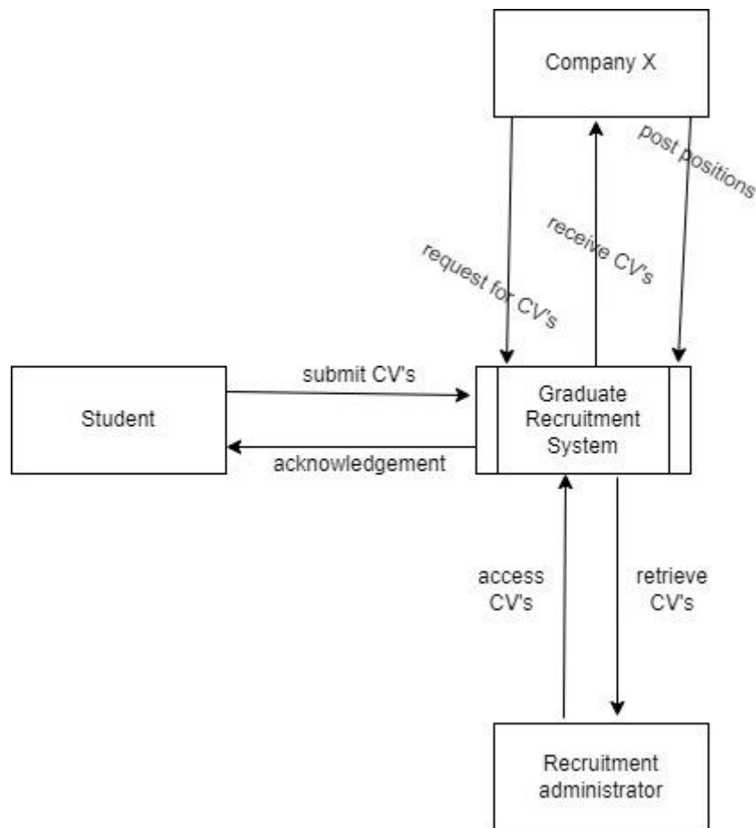
Figure 1: Context based dataflow diagram – Level 0
